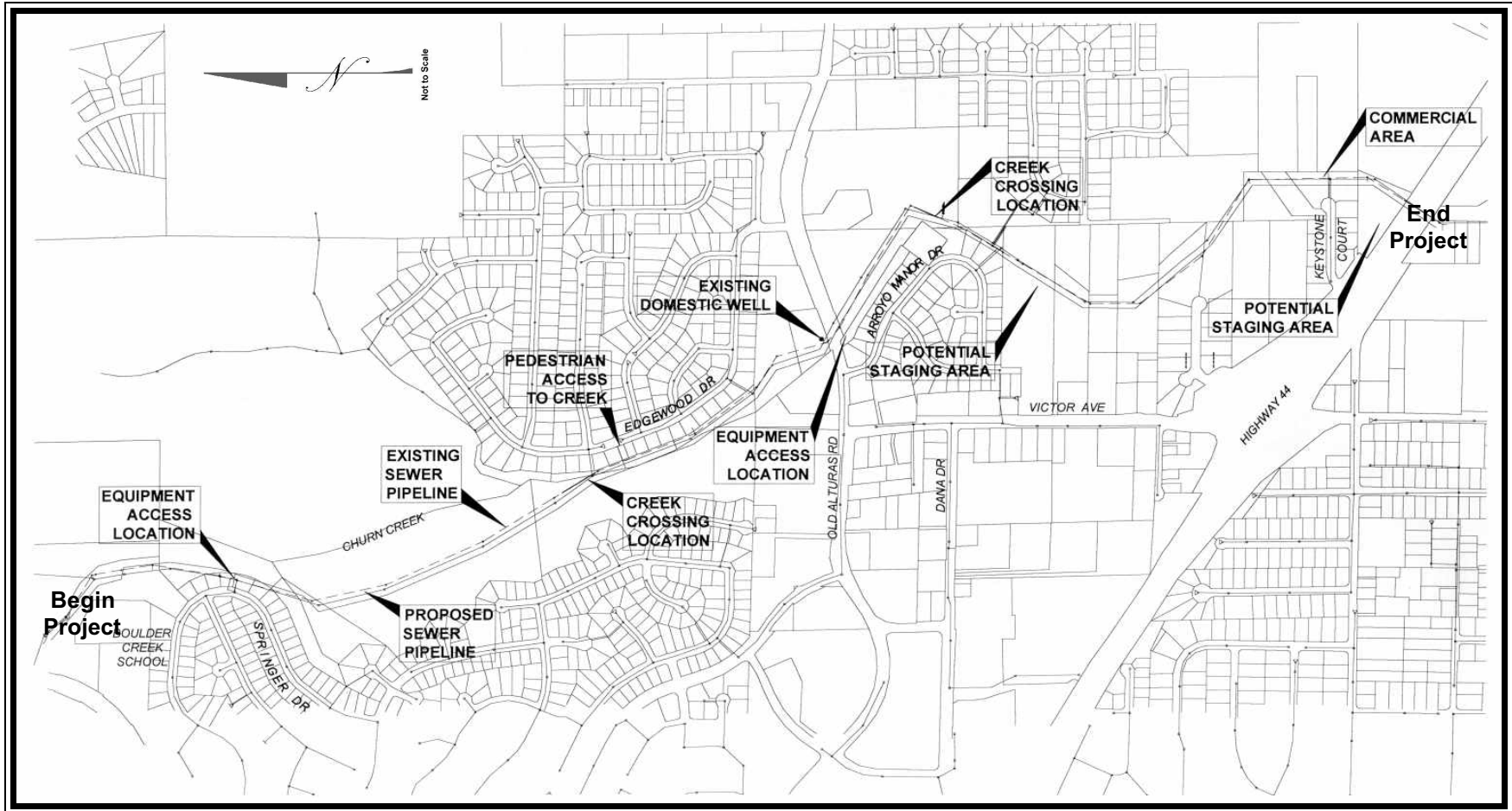
FIGURE 3-1 CITY OF REDDING EASTSIDE SANITARY SEWER INTERCEPTOR PROJECT FEATURES
